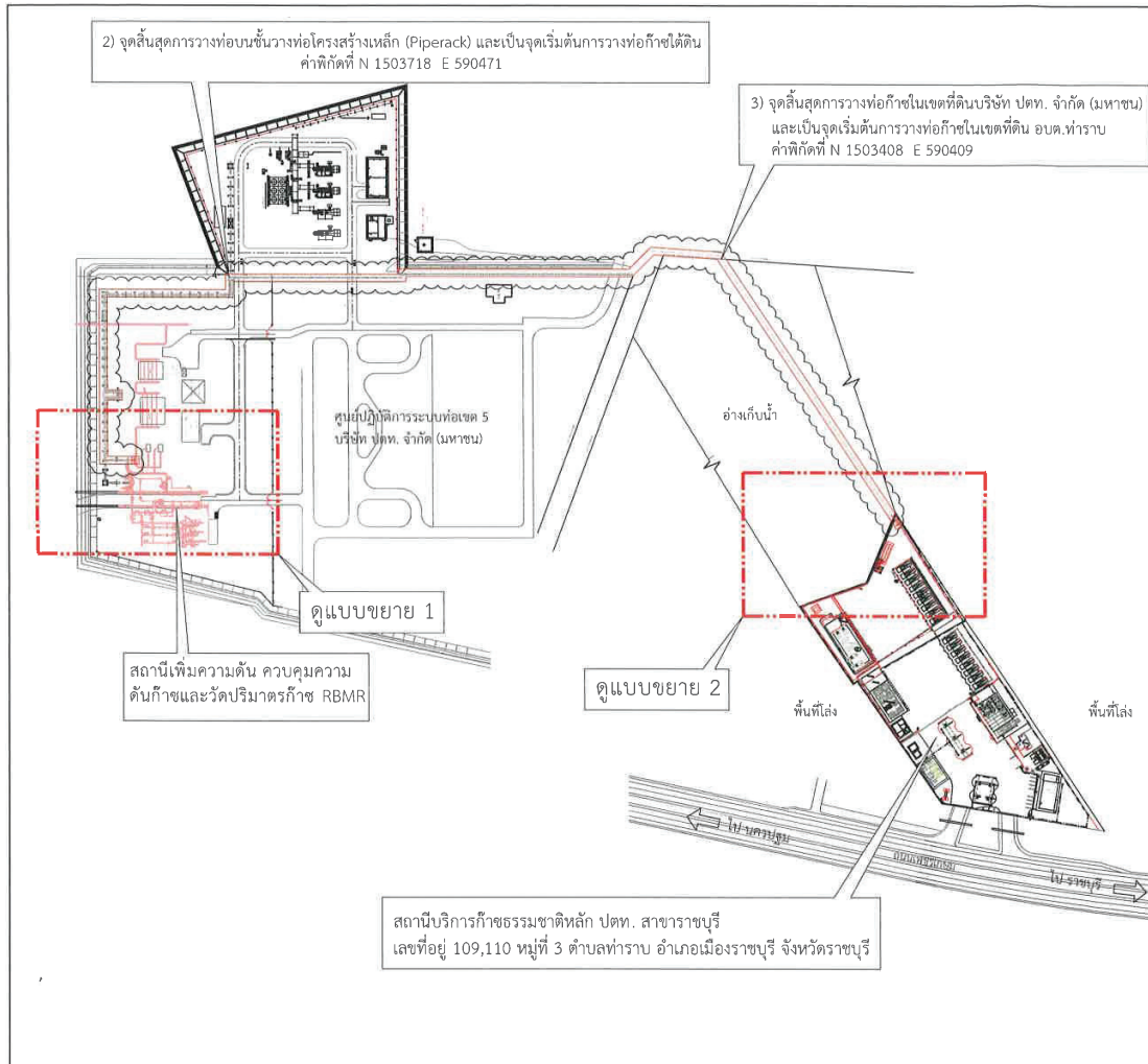
Plot Plan
