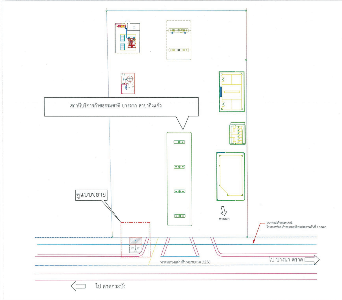
Plot Plan
