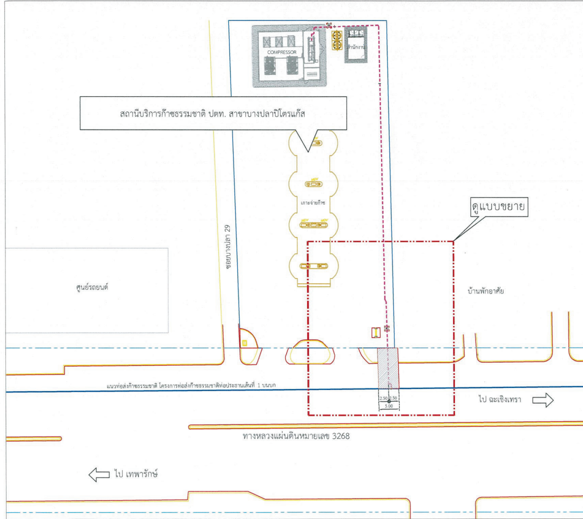
Plot Plan
